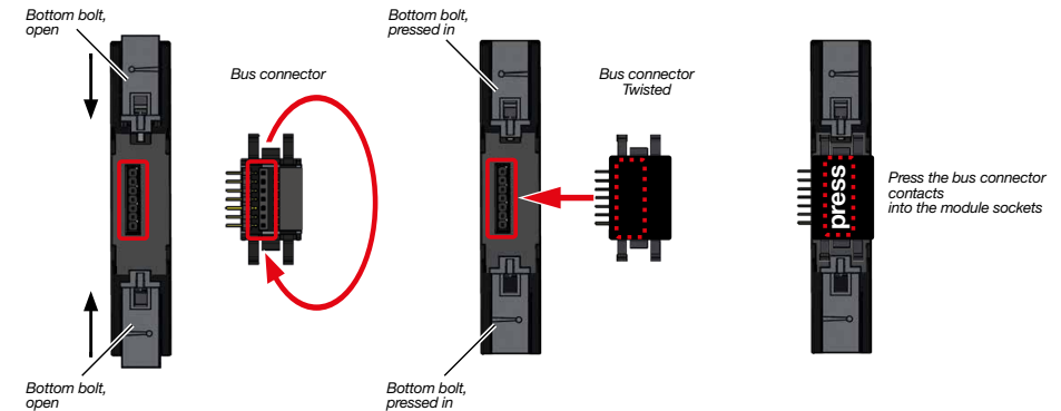
Fig.: Module rear views (without connection terminals)
