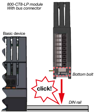
Fig.: Side view of the basic device and 800-CT8-LP module
