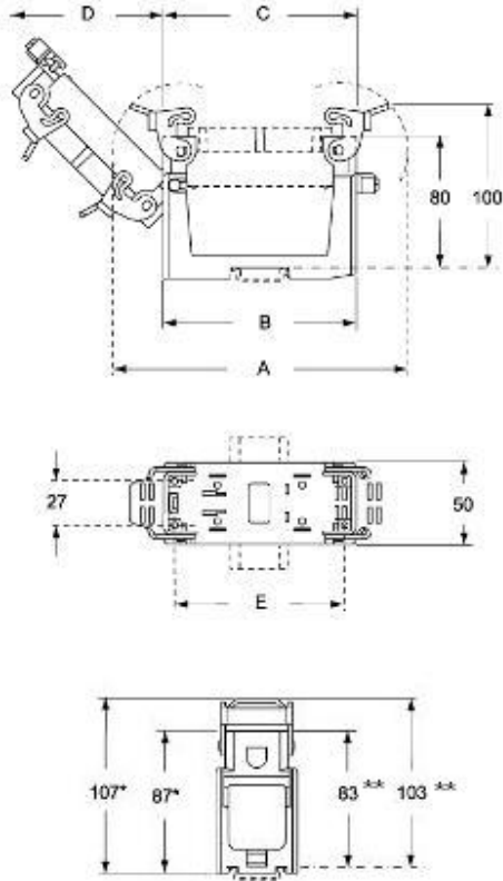
Catalogue drawings
