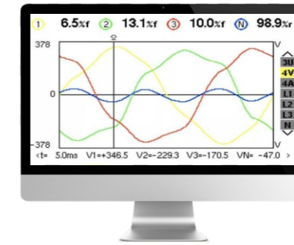
Before THDu governance
