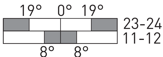
Switching diagram
