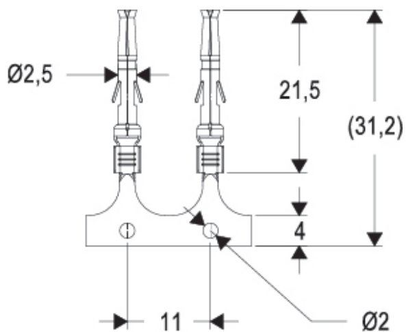
Catalogue drawings
