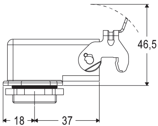
Catalogue drawings
