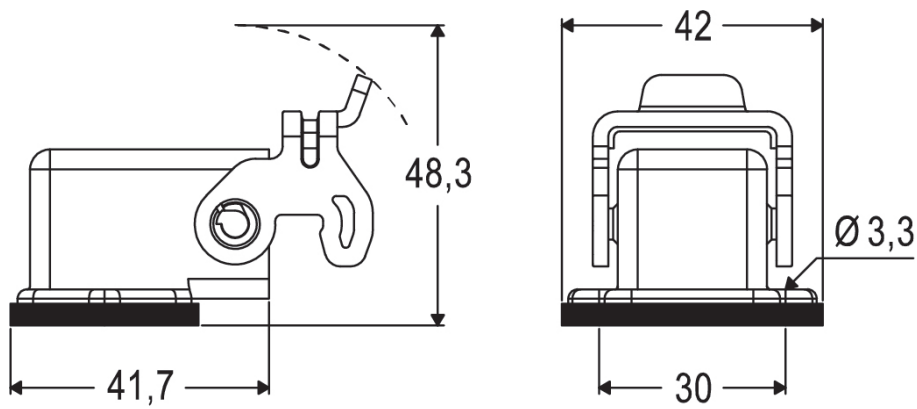
Catalogue drawings
